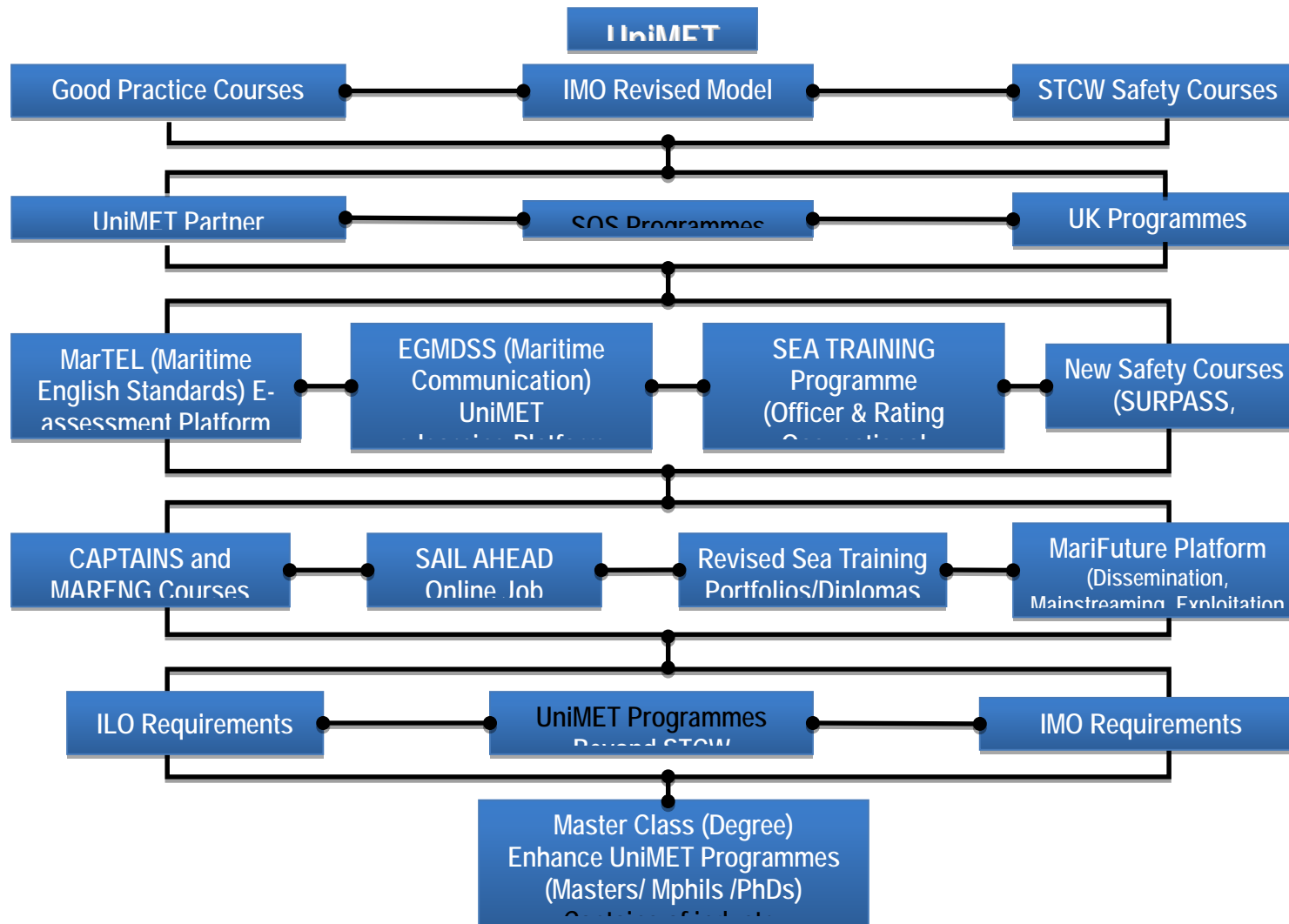
Figure 2 – UniMET Framework
